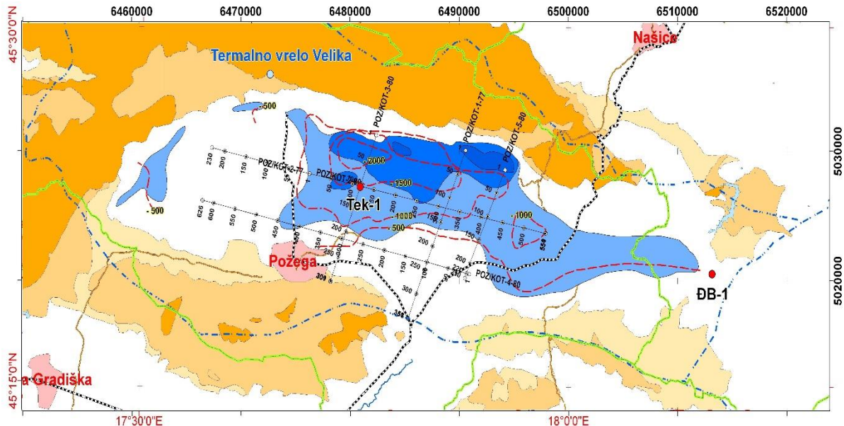
Figure 4. Interpretation based on 2D seismic profile and deep well Tek-1, potential favorable distribution of potential geothermal aquifers in carbonate rock masses (lighter shrubs) and bottom bridge sand (dark shrubs)
