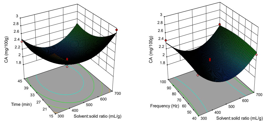
Figure 3. 3D plot showing the combined effects of HVED assisted extraction process on chlorogenic acid content of dust.
