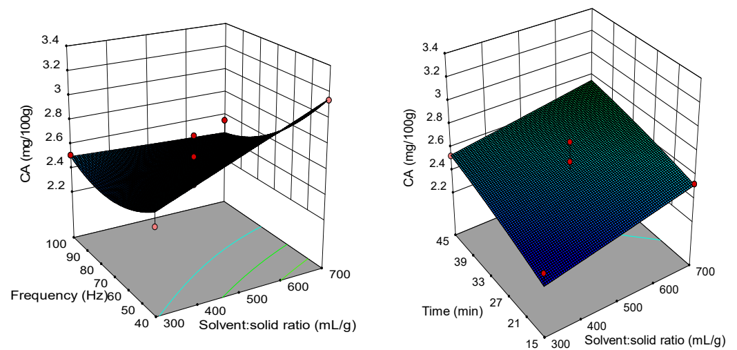
Figure 4. 3D plot showing the combined effects of HVED assisted extraction process on chlorogenic acid content of midrib.
