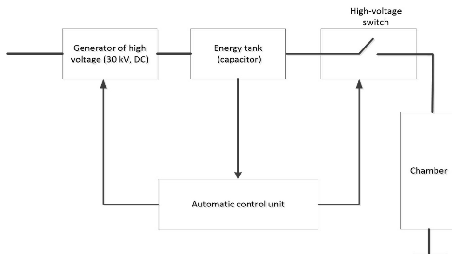
Figure 1. Scheme of HVED generator [20].
